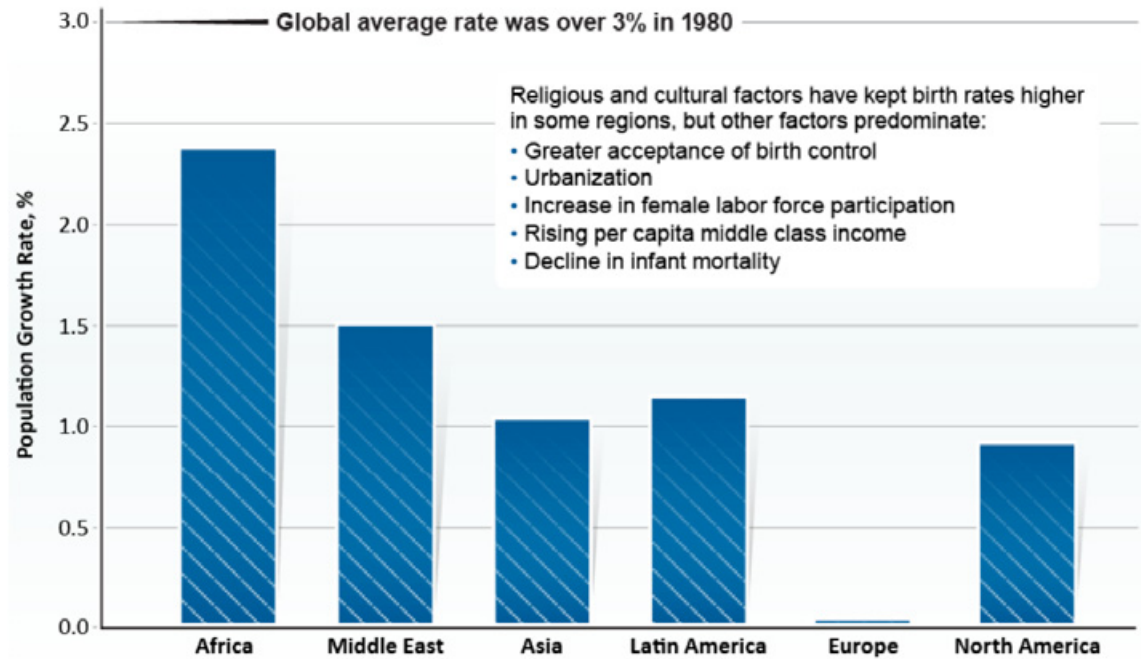
Figure 1 Global Population Changes in 2012.
